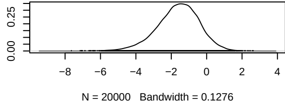
Density of d.Osimertinib.Placebo
