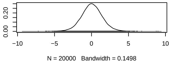
Density of d.Erlotinib.DHFRi
